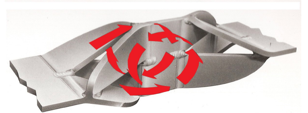
Counter-Rotating Vortices
