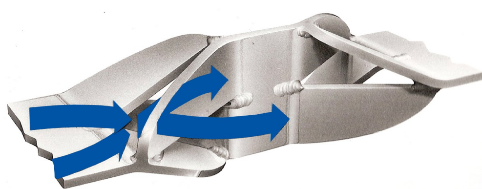
Cross-Current Mixing
